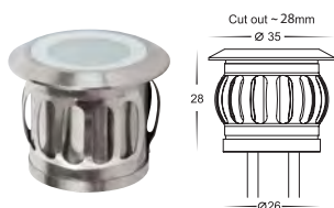
6 Light kit HV2826RGCW
