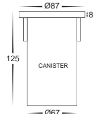
Cutout with Canister Ø87
