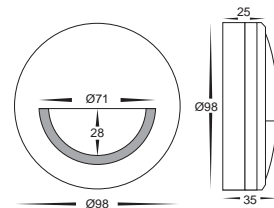
HV2961-TTM Aluminium Titanium
