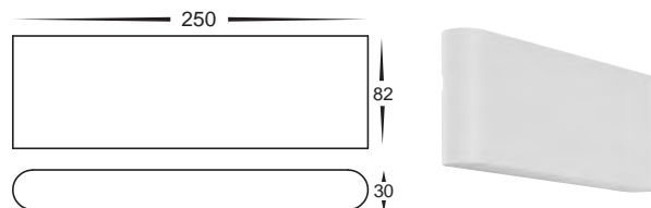
Fixed Down HV3652T-WHT-240V HV3652T-WHT-12V Aluminium White
