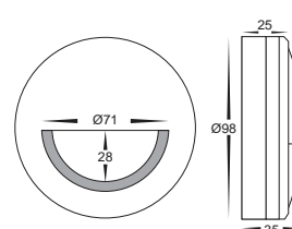
HV2961-BLK Aluminium Black
