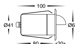
Cut Out Without Canister Ø42
