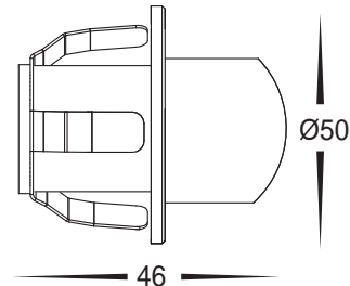
Cutout Ø30
