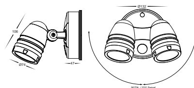
HV3794T-WHT (with sensor)
