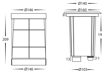
Cutout with Canister Ø146 Cutout without Canister Ø140
