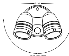
HV3794T-BLK (with sensor)
