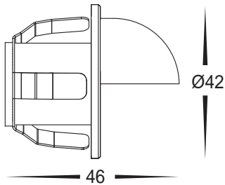
Cutout Ø30
