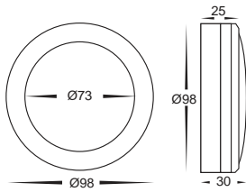
HV2960-TTM Aluminium Titanium
