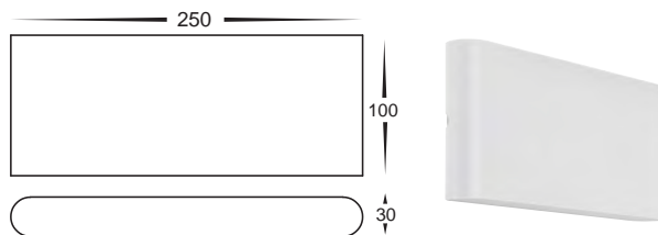
Up & Down HV3653T-WHT-240V HV3653T-WHT-12V Aluminium White
