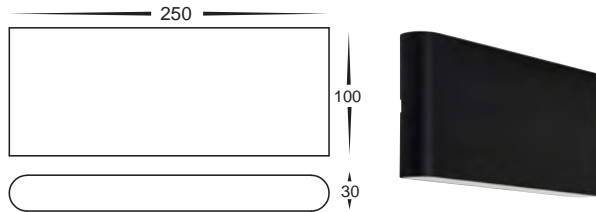
Up & Down HV3653T-BLK-240V HV3653T-BLK-12V Aluminium Black
