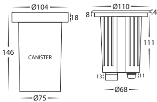
Cutout with Canister Ø104 Cutout without Canister Ø98
