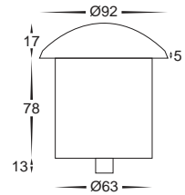
Cutout with Canister Ø87
