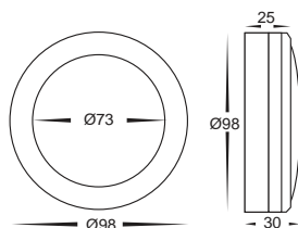
HV2960-BLK Aluminium Black
