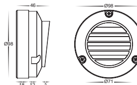
HV2925T-WHT-12V Aluminium White
