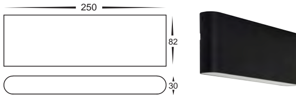
Fixed Down HV3652T-BLK-240V HV3652T-BLK-12V Aluminium Black
